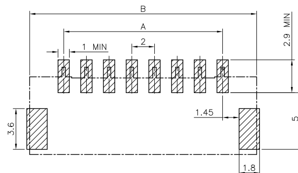
Recommended P.C.B LAYOUT General Tolerance \pm 0.05
